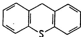
Thioxanthene
